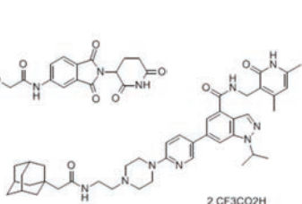
MS1943 trifluoroacetate
