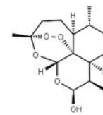
Dihydroartemisinin
