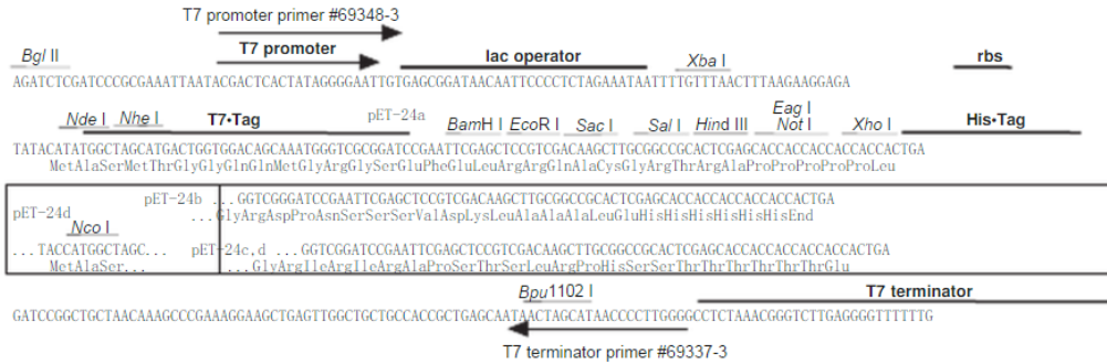
pET-24a-d(+) cloning/expression region
