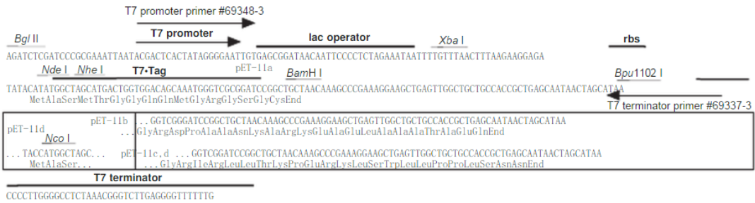
pET-11a-d cloning/expression region
