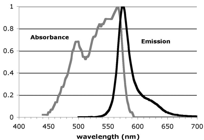
R-PE spectral properties
