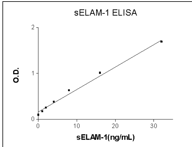
ELAM-1 Standard curve ranging from 1 to 32 ng/mL
