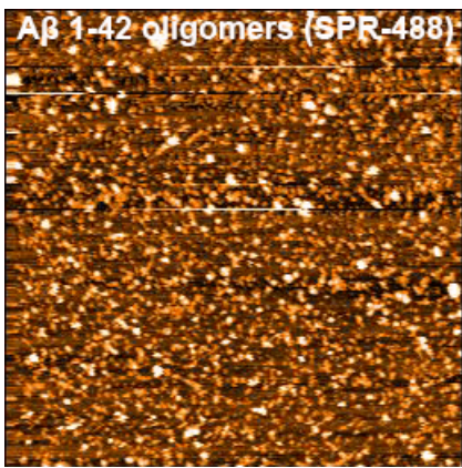
AFM of amyloid beta 1-42 oligomers (SPR-488). Atomic force microscopy analysis of 1.0 mg/mL samples diluted to 0.1 mg/mL in dH 2 O, mounted on freshly cleaved mica, washed, dried and analyzed with tapping mode. Representative images are 2.5 x 2.5 μm x-y with a z-range of 10 nm.
