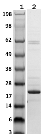
Coomassie stained SDS PAGE analysis of 30 µg HGPX2 product Lane 1: Molecular weight marker (SeeBlue™ Plus2) Lane 2: HGPX2
