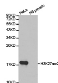
Western blot analysis of extracts of HeLa cell line and H3 protein expressed in E.coli., using H3K27me2antibody.
