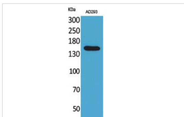
Western Blot analysis of AD293 cells using NTE Polyclonal Antibody.
