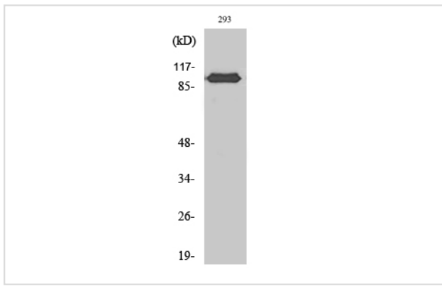
Western Blot analysis of 293 cells using CAS Polyclonal Antibody
