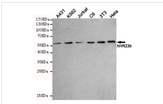
Western blot detection of hHR23b in A431, K562, Jurkat, C6, 3T3 and HeLa cell lysates using hHR23b antibody (1:1000 diluted). Predicted band size: 58 kDa. Observed band size: 58 kDa. Exposure time: 5 min.
