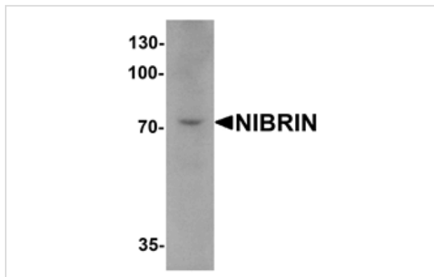
Western blot analysis of NIBRIN in mouse lung tissue lysate with NIBRIN antibody at 1 ug/ml.
