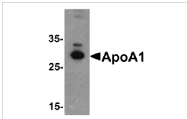
Western blot analysis of ApoA1 in chicken liver tissue lysate with ApoA1 antibody at 1 ug/mL .
