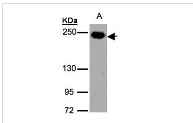
Sample(30 ug whole cell lysate) A: H1299 5% SDS PAGE Primary antibody diluted at 1: 1000
