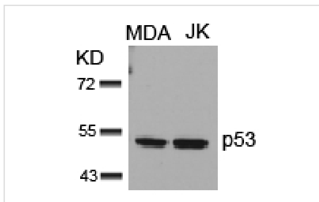
Western blot analysis of extracts from MDA and JK cells using p53(Ab-15) Antibody #21085.
