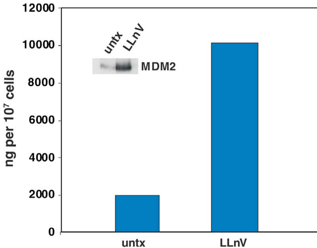
Figure 2: Lysates prepared from U2OS human osteosarcoma +/- LLnV cells were quantified with this DuoSet IC. The same lysates were also immunoblotted (inset) with a monoclonal detection antibody. The DuoSet IC results correlate well with the relative amounts of MDM2 detected by Western blot.
