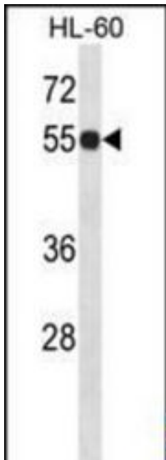
IMPDH1 Antibody (N-term) Western blot of HL-60 cell line lysates (35 ug/lane). This demonstrates the IMPDH1 antibody detected the IMPDH1 protein (arrow).
