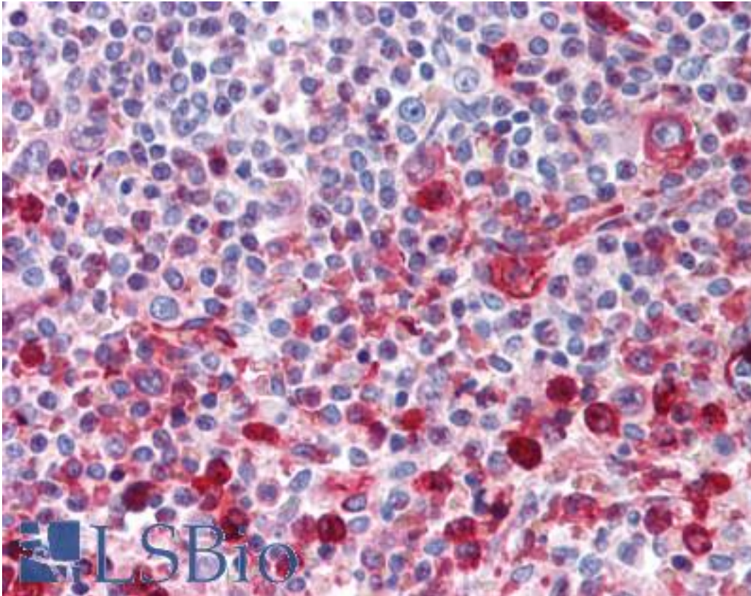
Anti-WNT16 antibody LS-A9630 IHC of human spleen. Immunohistochemistry of formalin-fixed, paraffin-embedded tissue after heat-induced antigen retrieval.
