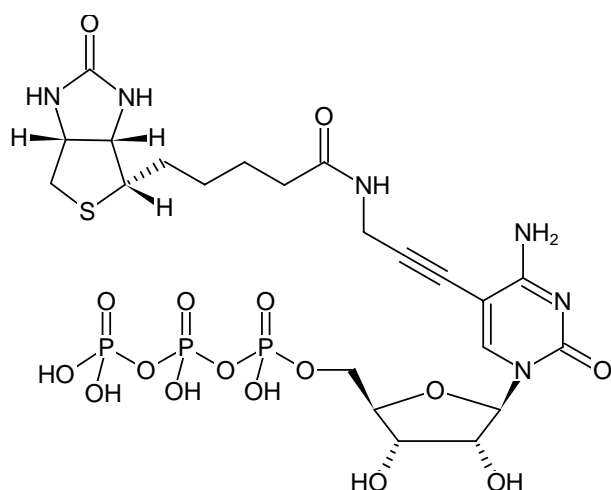
Structural formula of Biotin-4-CTP
