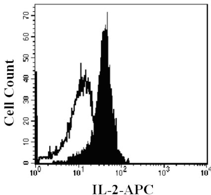
Intracellular staining of LPS-stimulated porcine PBMCs with APC-conjugated anti-porcine IL-2 (Catalog # IC6521A, filled histogram) or with APC-conjugated isotype control antibody (Catalog # IC0041A, open histogram).
